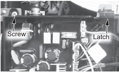
Figure 20 - Control board location
